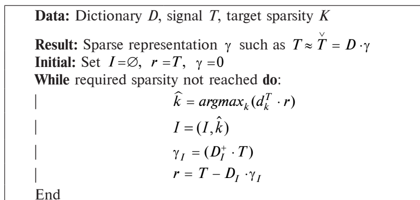
Fig. 1. OMP algorithm based on [2]
