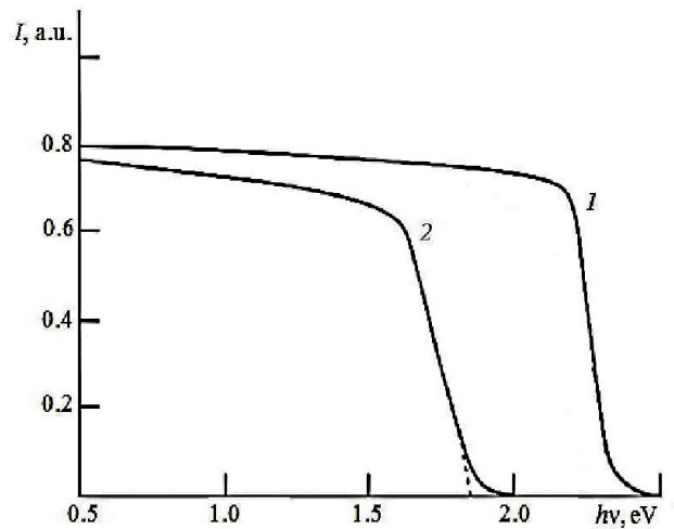
Fig. 2. Optical absorption spectra of GaP(111) (1) and GaP(111) with the Ga 0.6 In 0.4 P nanofilm about 50 Å thick (2)
