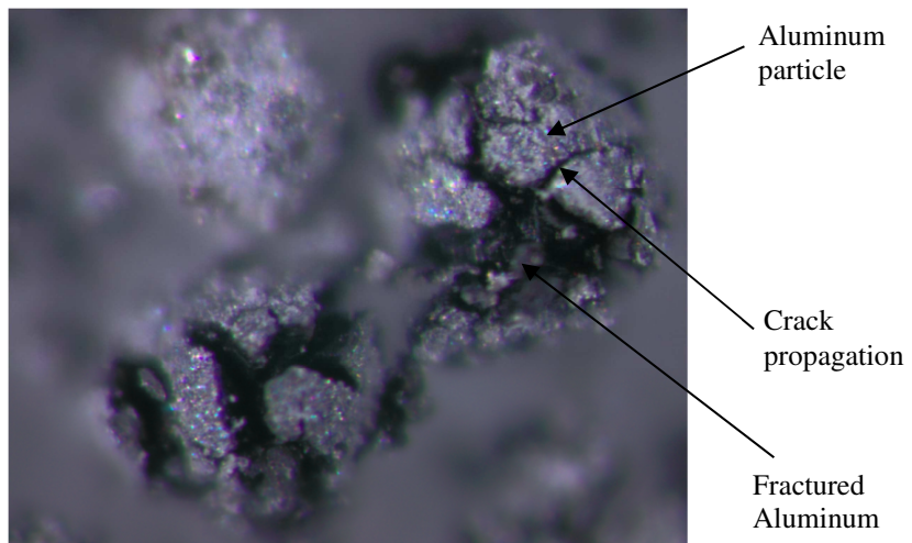
Fig. 1. Crack formation on the activated aluminum particles at \sim 30 °C.
