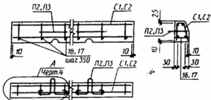
БР300.45.18 и БР300.60.20
