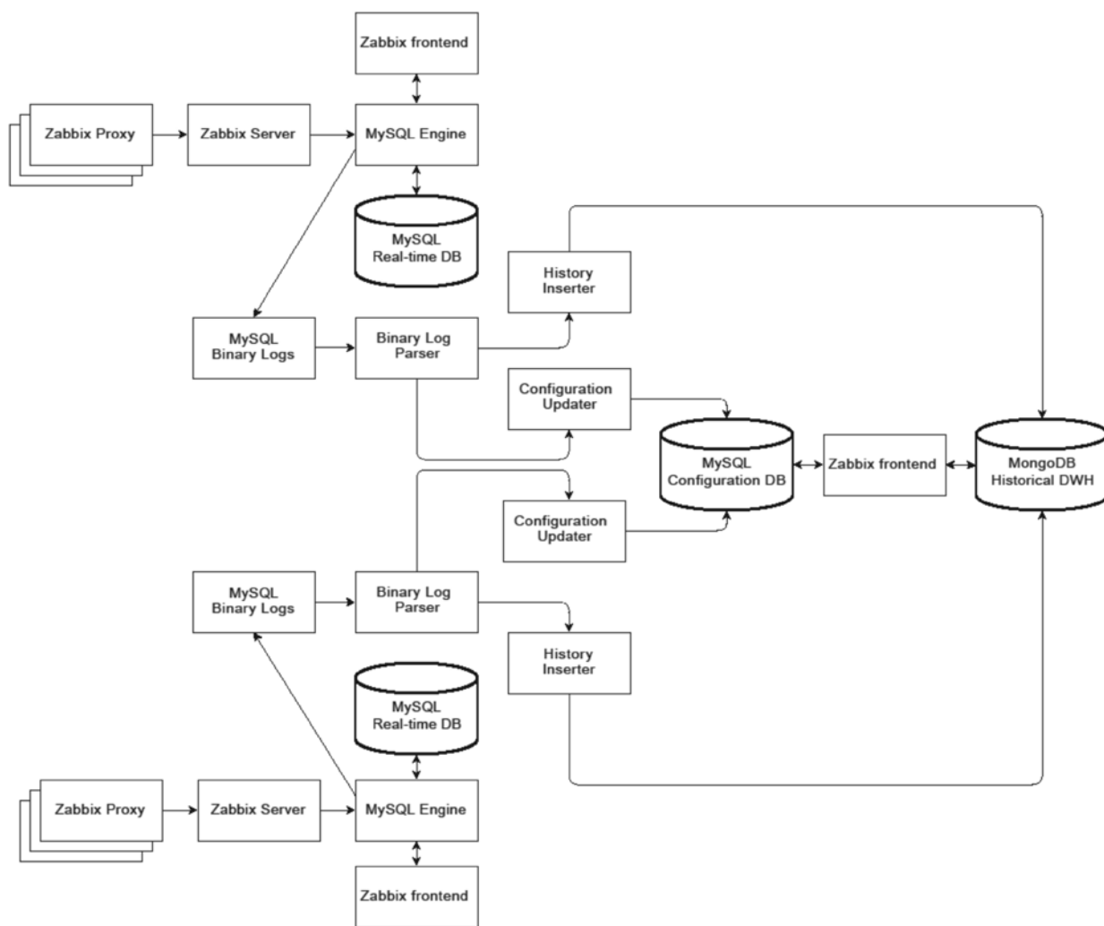
Fig. 4. Octopus Distributed Architecture
