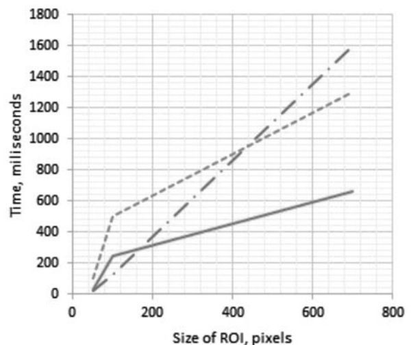
Fig. 4. Correspondence between computation time and the size of a ROI in relation to different values of the threshold in the SURF algorithm (- . -) threshold equals 400; (—) threshold equals 100; (- -) threshold equals 50
