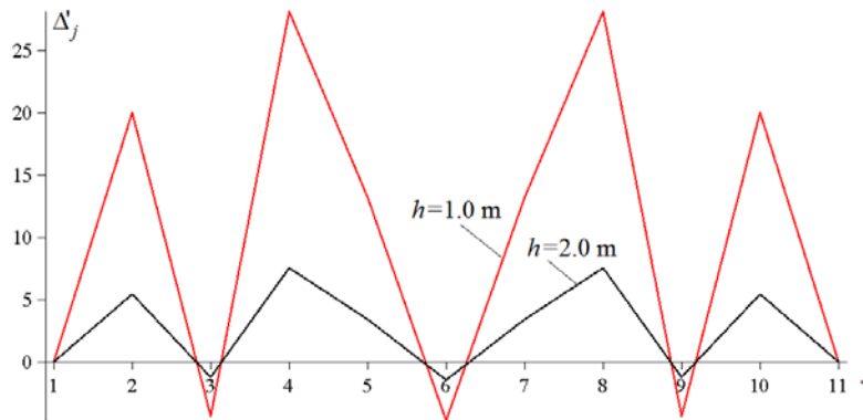
Figure 7. Displacements of the nodes in the lower truss chord. L=4na=100m, n=5, \Delta'_j = EF \Delta_j / (PL)
