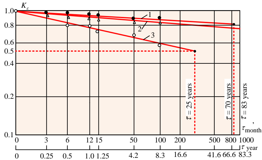
Figure 2. Change in the coefficient of aging of polymer membranes by breaking elongation in various conditions: 1 – under water at t = -20+30\text{ }^{\circ}\text{C} ; 2 – direct atmospheric exposure at t = -20+30\text{ }^{\circ}\text{C} ; 3 – a protective coating of ground with a thickness of 0.5 m at t = -15+20\text{ }^{\circ}\text{C} .
