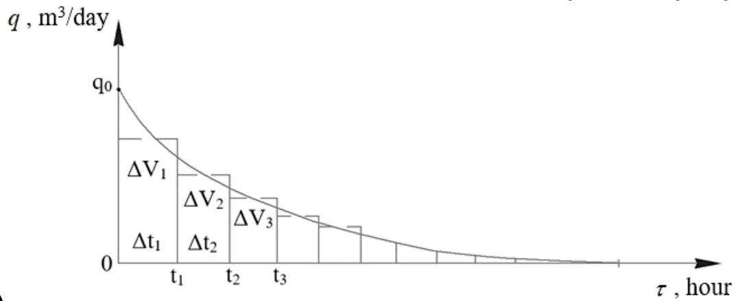
Figure 4. Scheme of water permeability of a bentomat screen with a protective layer of ground under conditions of damage self-healing:
