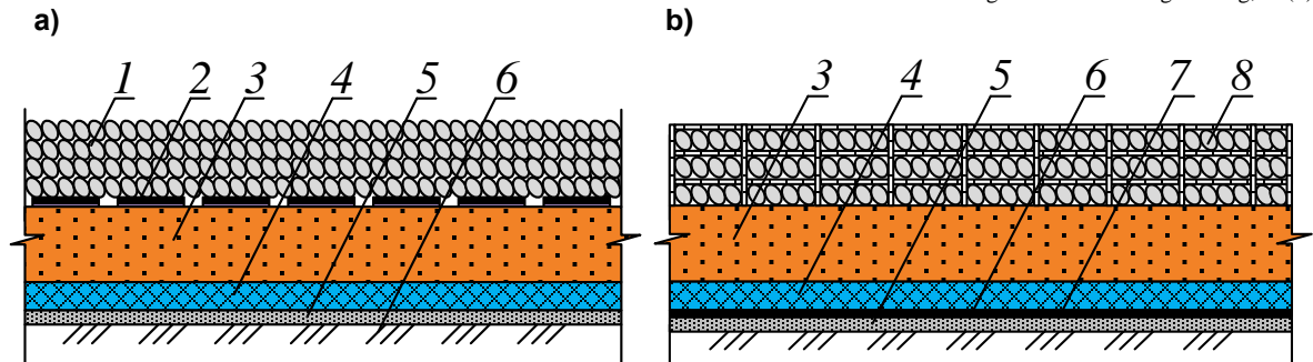
Figure 1. Multilayer constructions of seepage-control coatings with geosynthetics for canals and ponds: a, b – with a seepage-control element made of bentonite mats and a protective layer; 1 – a protective coating of rockfill; 2 – non-woven geotextile; 3 – a protective layer of ground; 4 – bentonite mat; 5 – the underlying layer of sand; 6 – compacted base; 7 – polymer geomembrane thermally bonded with a lower layer of bentonite mat; 8 – gabions filled with rocks.
