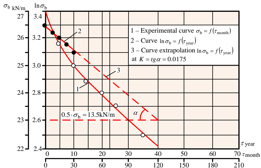
Figure 3. Diagram of changes of geomembrane strength at break depending on the time of observation.
