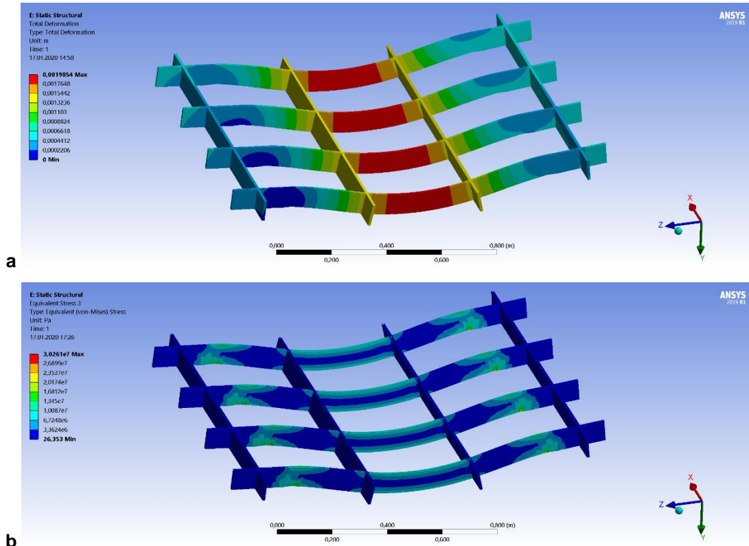
Figure 11. Deformations (a) and von-mises Stress (b) of pure wood frame T3.
