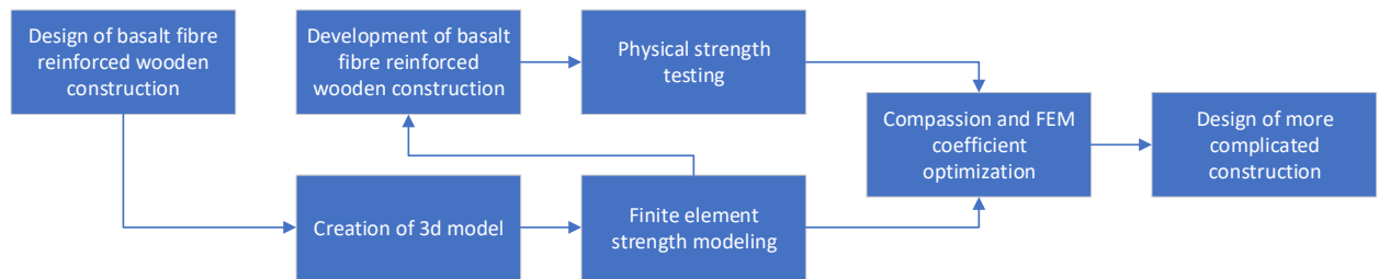
Figure 4. Research methodology.
