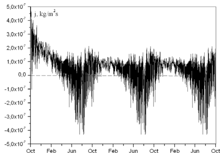
Figure 8. The density of diffusion moisture flow at the brickwork-insulation boundary.
