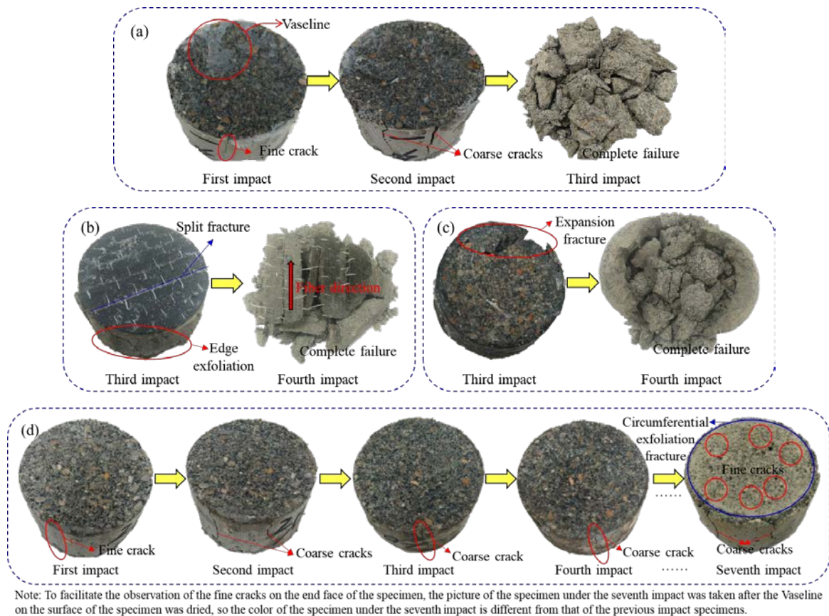
Figure 12. Cyclic impact failure states of specimens with four different confine conditions: (a) No-C; (b) CFRP-E-C; (c) CFRP-S-C; and (d) SC-S-C.
