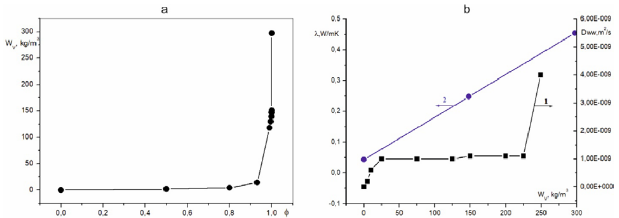
Figure3. Mineral wool a) moisture storage function, b) 1 – liquid transport coefficient, 2 – thermal conductivity.
