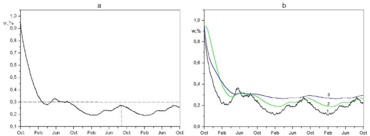
Figure 13. Relative humidity of brickwork at external facing resistance to vapor permeability S_d = 0.5 m: a) average, b) 1 – outer layer, 2 – middle layer, 3 – inner layer.
