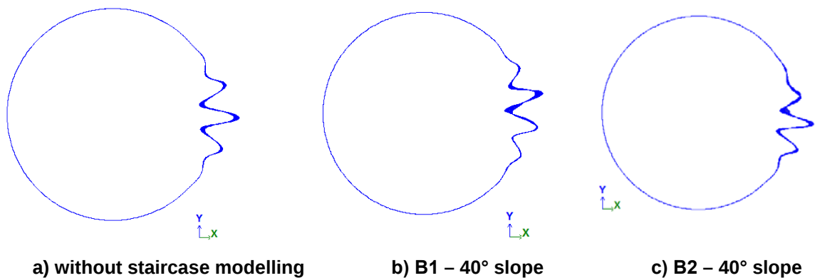
Figure 9. The shape of the loss of rigidity of the shell of the tank with a volume of 20 thousand m^3 at the level of +9.000 m.
