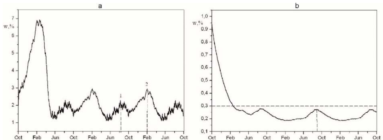
Figure 10. Relative mass humidity at external facing resistance to vapor permeability Sd = 0.2 \text{ m} : a) mineral wool, 1, 2 – annual humidity maxima; b) brickwork.
