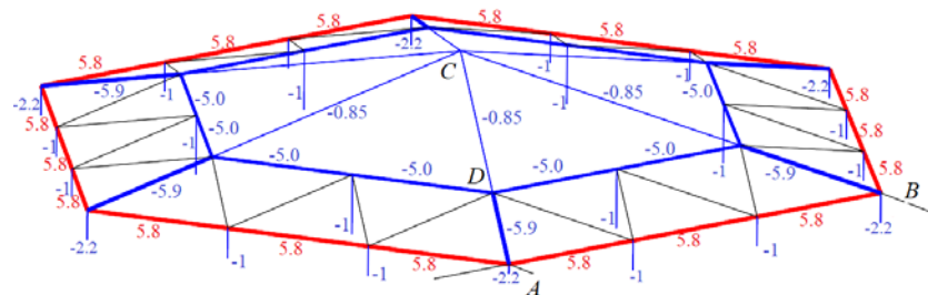
Figure 4. Distribution of forces in the rods, n=3 , a=5.0 m, h=1.0 m.
