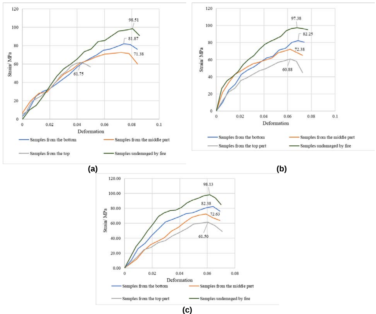
Figure 7. The strength of pinewood weakened by fire in tension along the fibers in different parts of the trunk: (a) Namsky Appany; (b) Namtsy-1 Khomustakh; (c) Namsky Edeytsy (Yakutia, Russia).
