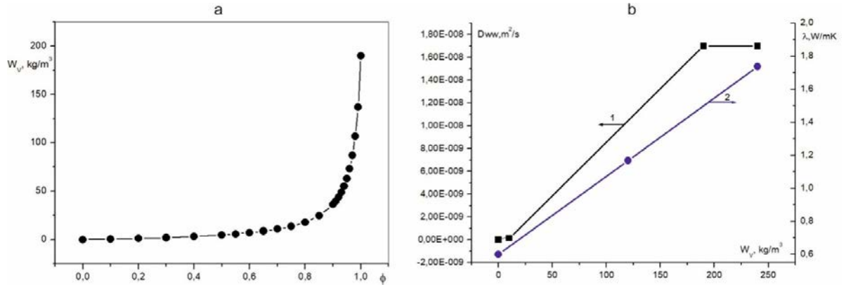
Figure2. Brickwork a) moisture storage function, b) 1 – liquid transport coefficient, 2 – thermal conductivity.
