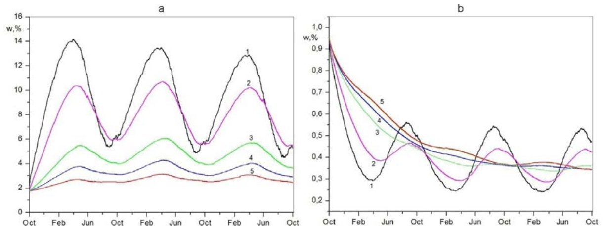
Figure16. A change in relative mass humidity of a) mineral wool and b) brickwork at facing resistance to vapor permeability S_d = 10 m and retarder resistance to vapor permeability: 1 – S_d = 0 m, 2 – 1 m, 3 – 5 m, 4 – 10 m, 5 – 20 m.
