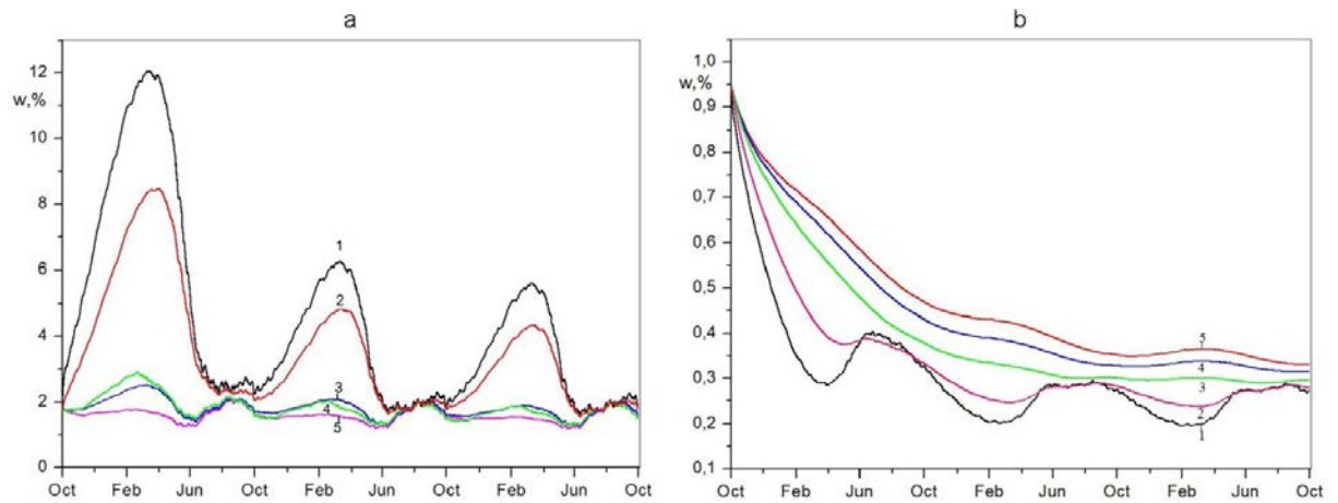
Figure15. A change in relative mass humidity of a) mineral wool and b) brickwork at facing resistance to vapor permeability S_d = 1 m and retarder resistance to vapor permeability: 1 – S_d = 0 m, 2 – 1 m, 3 – 5 m, 4 – 10 m, 5 – 20 m.
