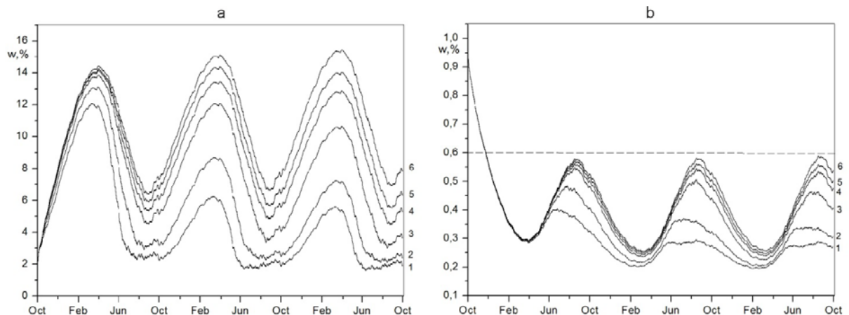
Figure 14. Relative mass humidity: a) mineral wool, b) brickwork at different resistances of facing to vapor permeability: 1 – S_d = 1 m, 2 – 2m, 3 – 5m, 4 – 10m, 5 – 20m, 6 – impermeable.
