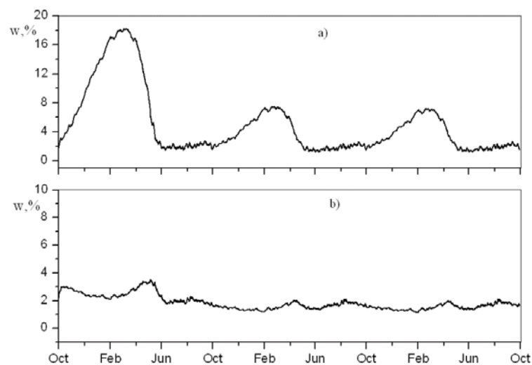
Figure 12. Average relative humidity of mineral wool at external facing resistance to vapor permeability Sd = 0.5 m over the layers: a) outer half, b) inner half.
