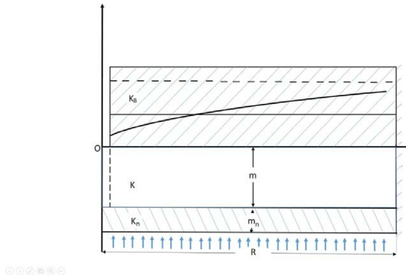
Figure 1. Schematic model of the flow in the three-layer porous medium.
