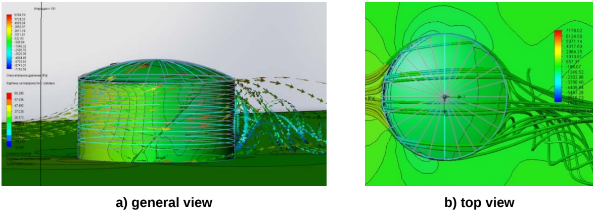
Figure 5. Model in SolidWorks for wind pressure calculation.
