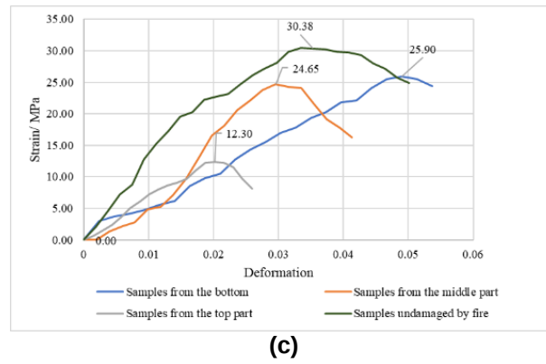
Figure 6. The strength of pinewood weakened by fire for compression along the fibers in different parts of the trunk: (a) Namsky Appany; (b) Namtsy-1 Khomustakh; (c) Namsky Edeytsy (Yakutia, Russia).
