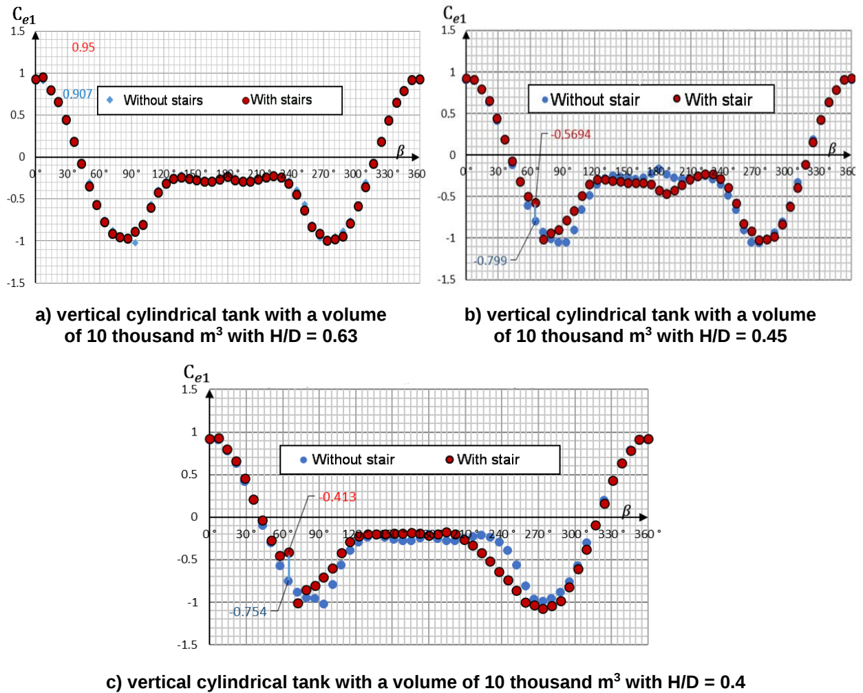
Figure 11. Improved aerodynamic coefficients for a tank with a spiral staircase.
