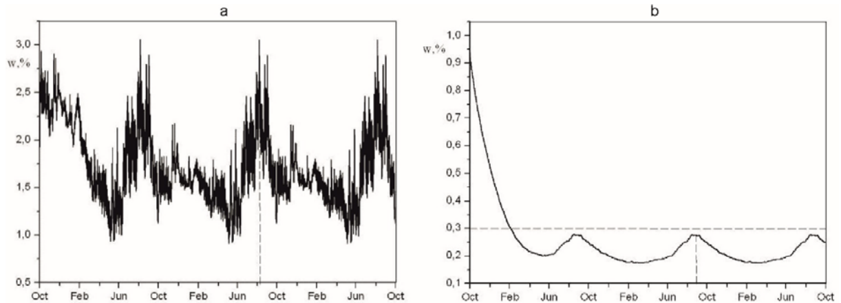
Figure 7. Relative mass humidity without external facing: a) mineral wool, b) brickwork.
