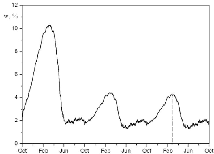
Figure 11. Average relative humidity of mineral wool at external facing resistance to vapor permeability Sd = 0.5 m.
