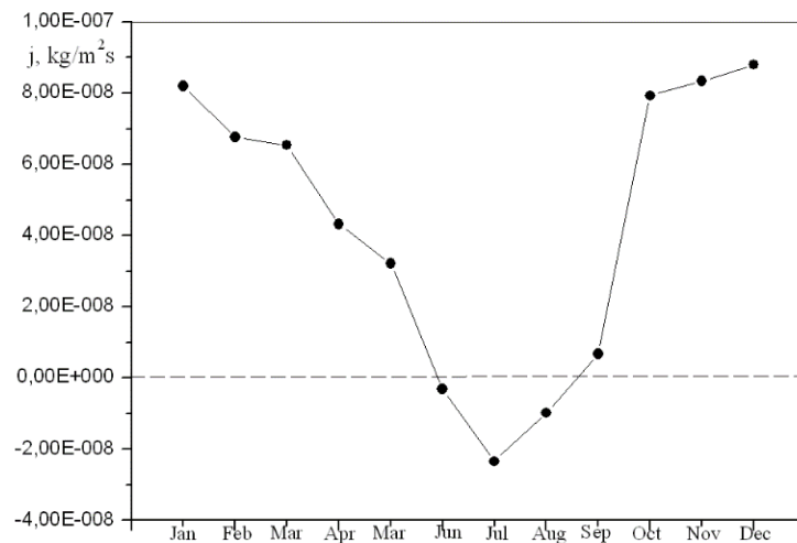
Figure 9. The average monthly density of the diffusion moisture flow at the brickwork-insulation boundary.
