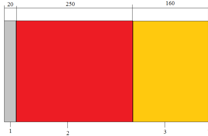
Figure1. The outer wall composition: 1 – cement-sand plaster, 2 – brickwork, 3 – mineral wool insulation, 4 – outer facing.
