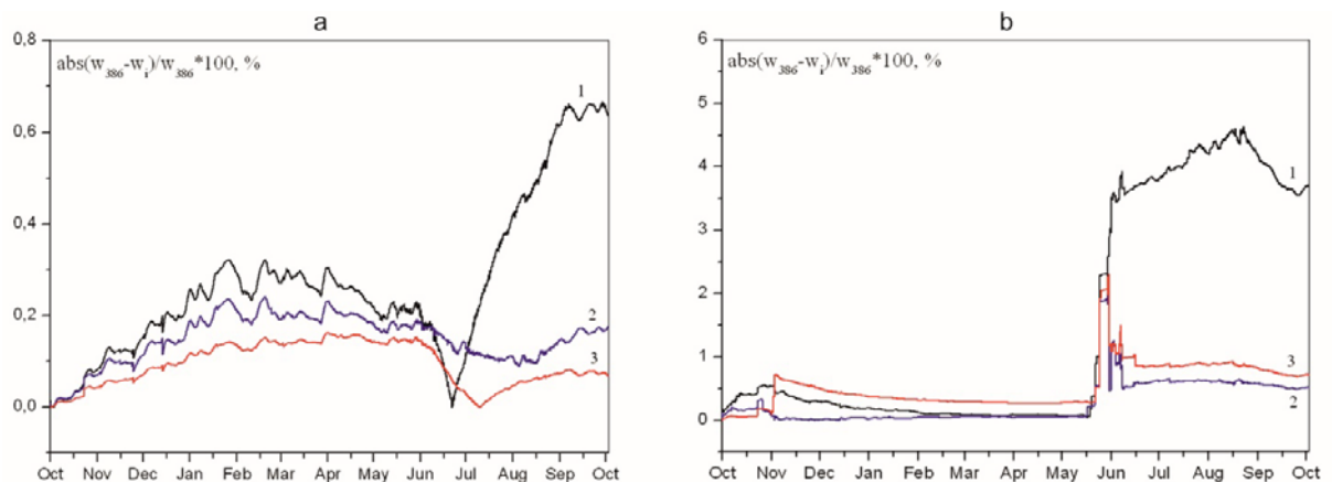
Figure 6. Comparison of average relative humidity for: a) brickwork, b) mineral wool with a different number of grid cells: 1 – i = 128 , 2 – 172, 3 – 258.
