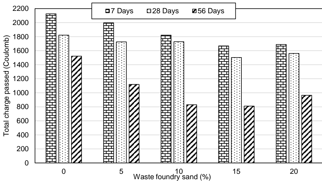
Figure 10. Total charge passed through concrete mixtures cured in 10% sulfate solution after initial water curing of 28 days.
