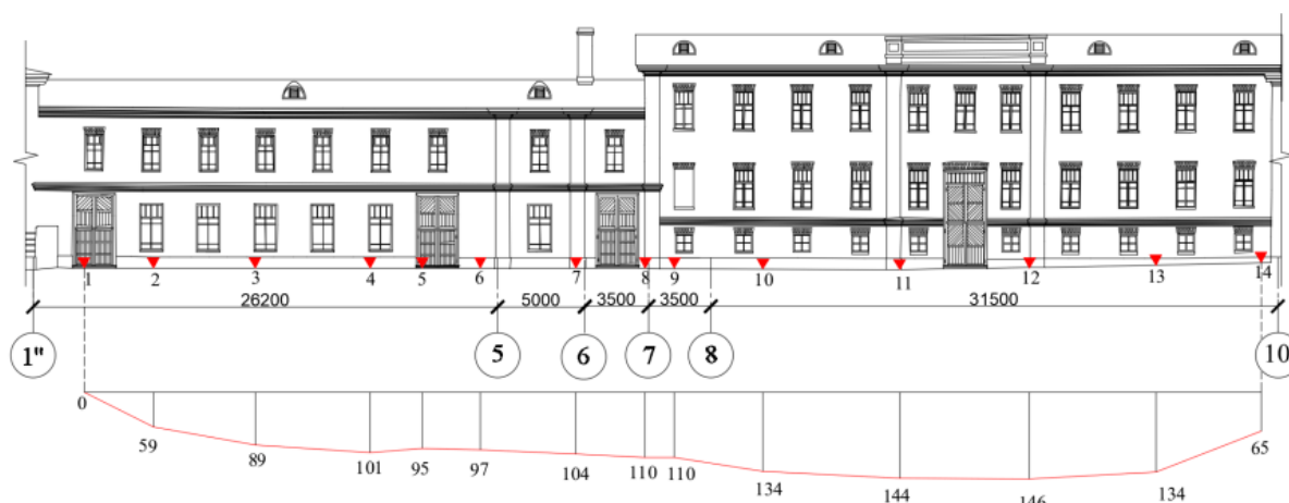
Figure 13. Diagram of the accumulated settlements across wall A. The values are given in millimeters 5 .
