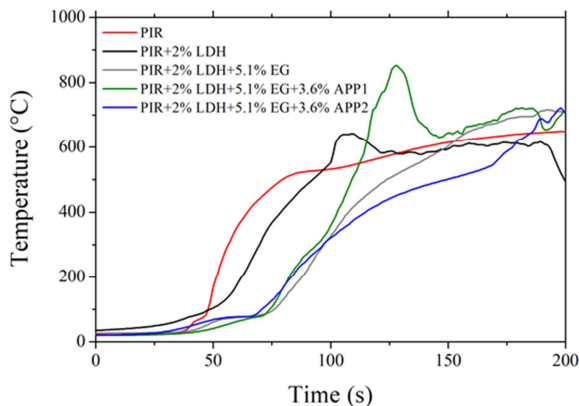
Fig. 6. Unexposed surface temperature of all formulations.
